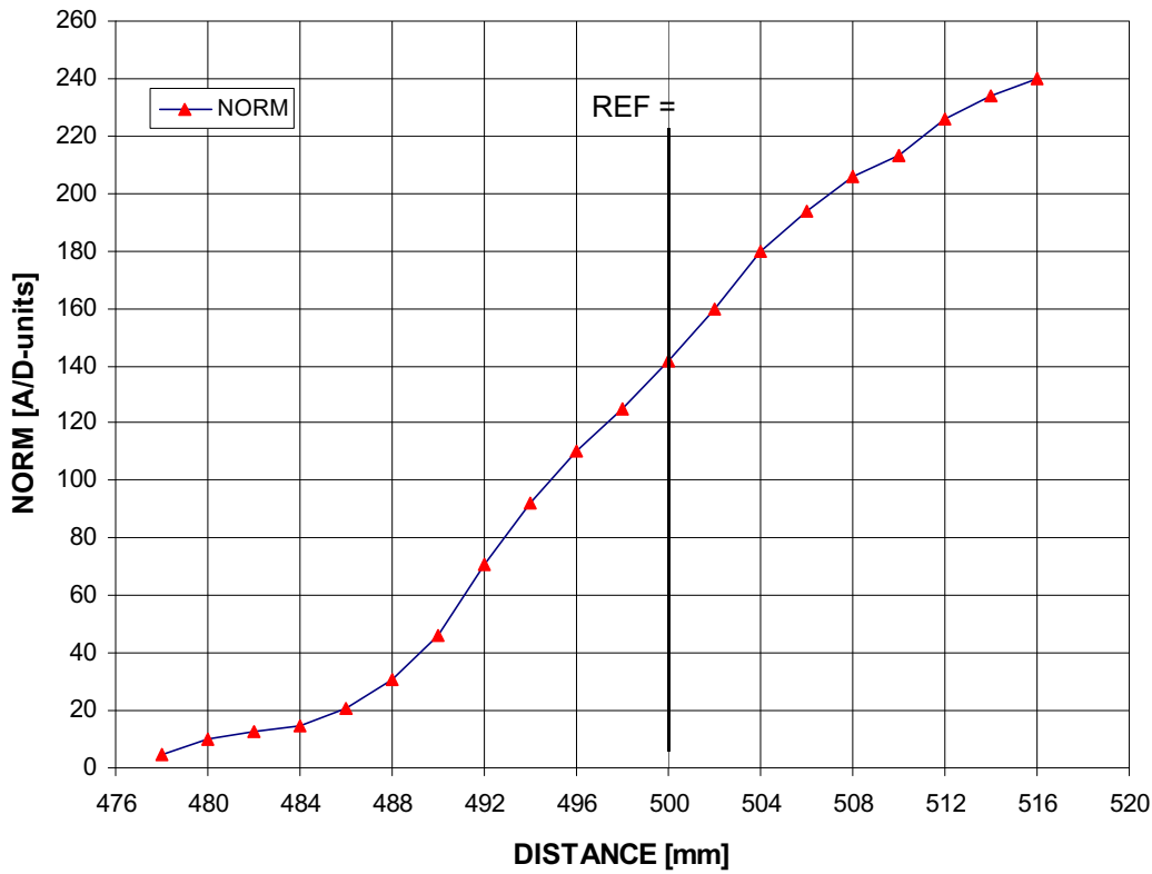
Characteristic Curve: R-LAS-LT-500 (Ser.No. 00877)
