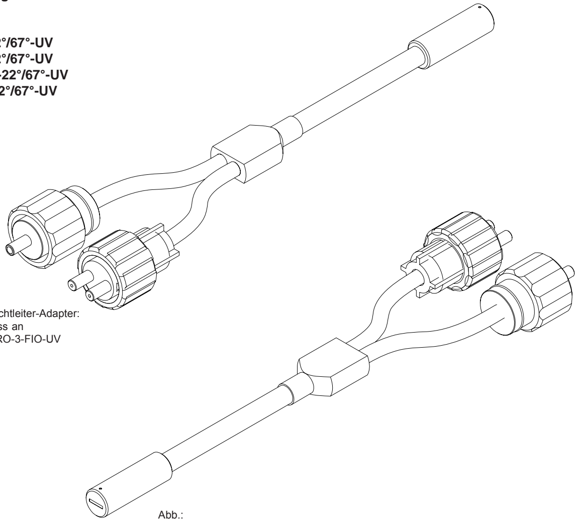
Abb.: R-S-R2.1-(6x1)-1200-Y-22°/67°-UV
