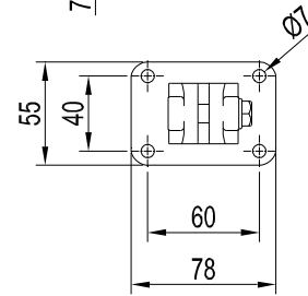
Flange clamp stainless steel (VA) FK 30
