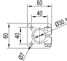
Foot clamp stainless steel (VA) FS 30
