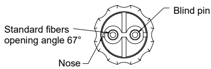
Reflected light fiber optics: R-S-A2.0-(2.5)-1200-67°-(1P+1BP) (with one blind pin)
